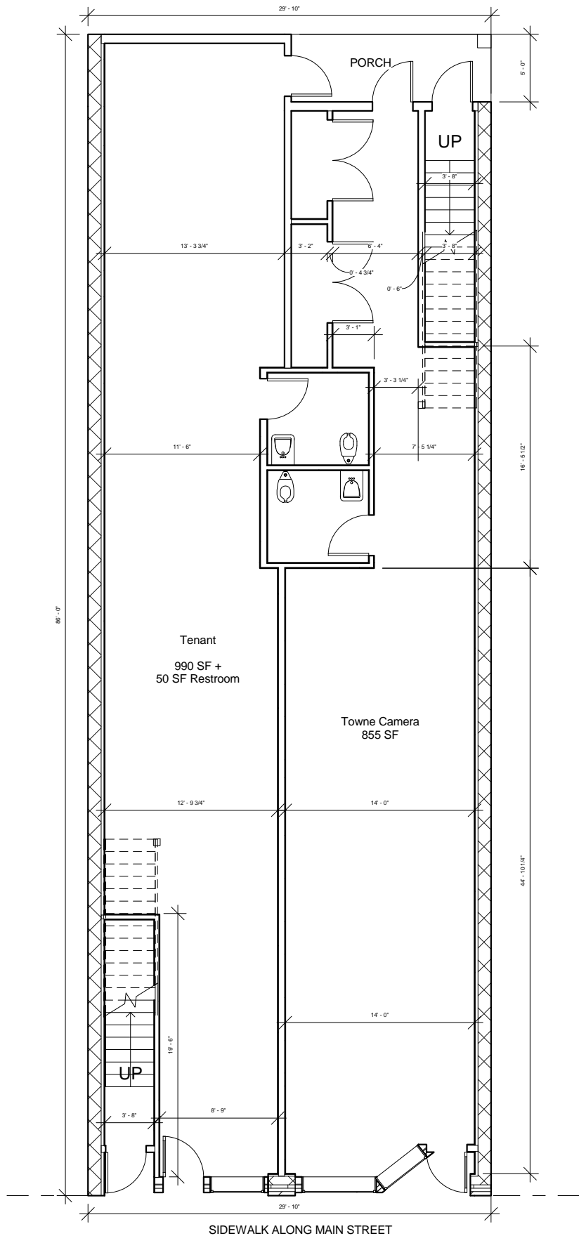
1 First Floor 1" = 10'-0"
